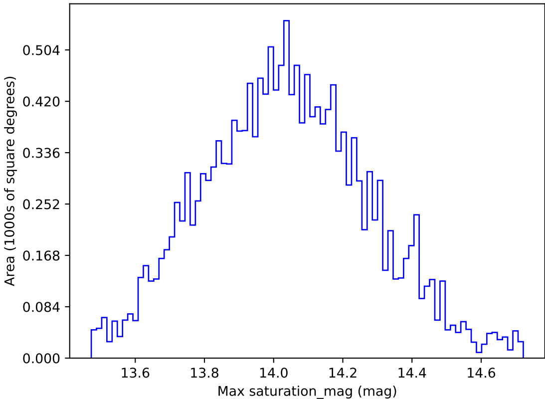
ddf_loaded_fl15_v3.4_10yrs WFD u band: Max saturation_mag
