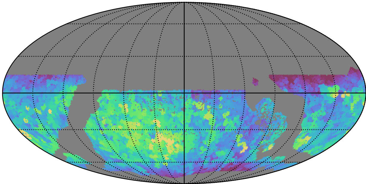
ddf_loaded_fl15_v3.4_10yrs WFD r band: Max saturation_mag
