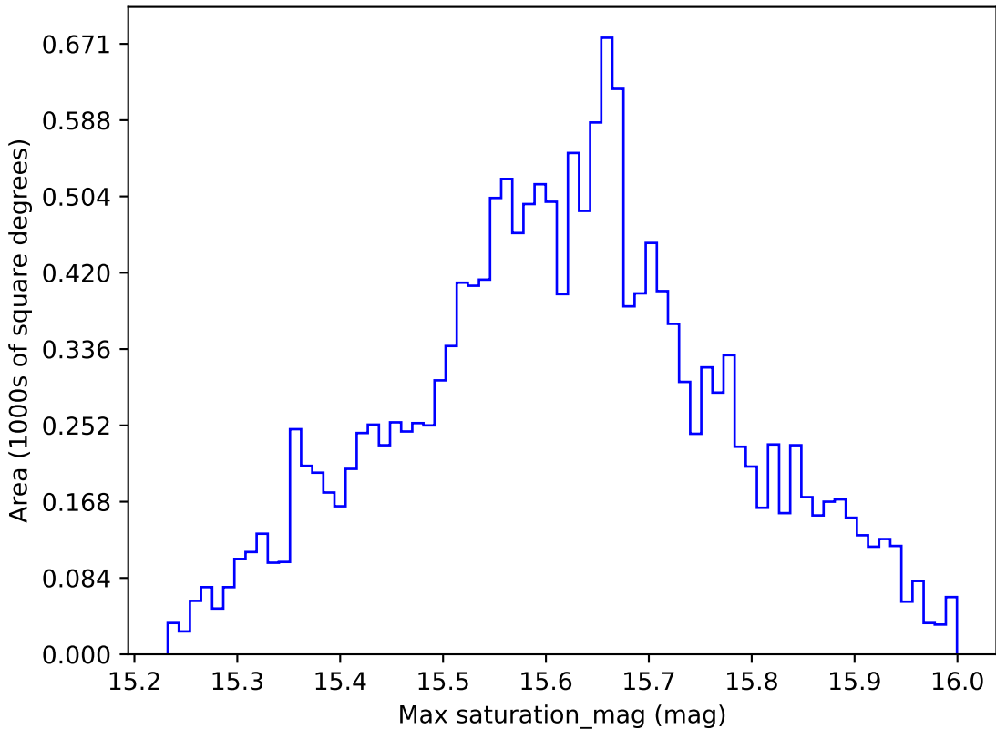
ddf_loaded_fl15_v3.4_10yrs WFD i band: Max saturation_mag
