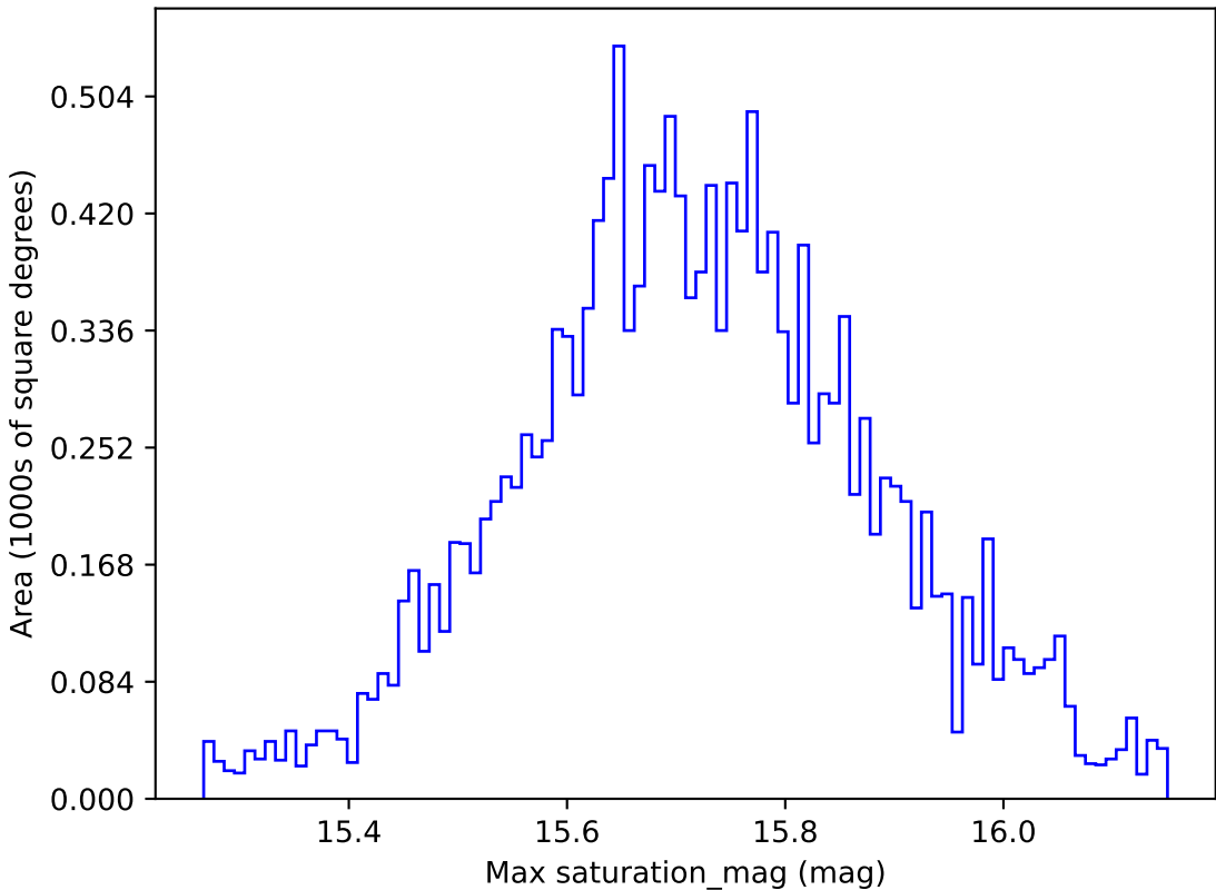
ddf_loaded_fl15_v3.4_10yrs WFD g band: Max saturation_mag
