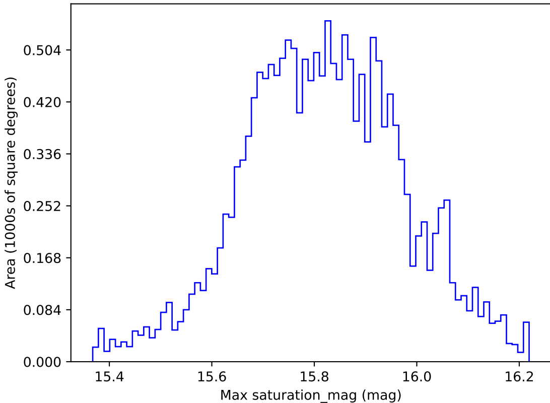
ddf_loaded_fl15_v3.4_10yrs WFD all bands: Max saturation_mag
