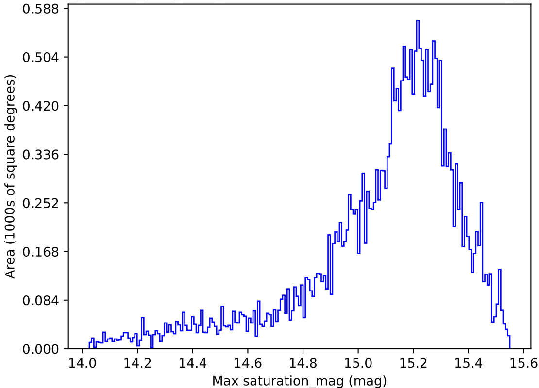
ddf_loaded_fl15_v3.4_10yrs All sky z band: Max saturation_mag
