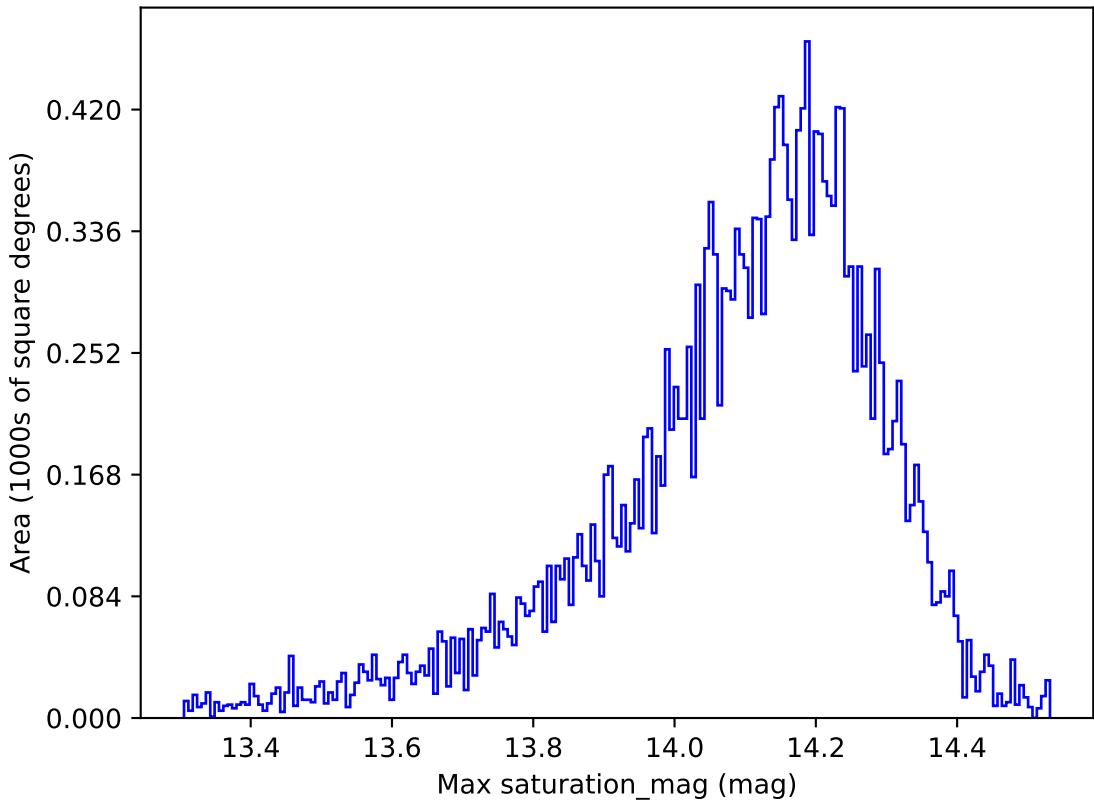
ddf_loaded_fl15_v3.4_10yrs All sky y band: Max saturation_mag
