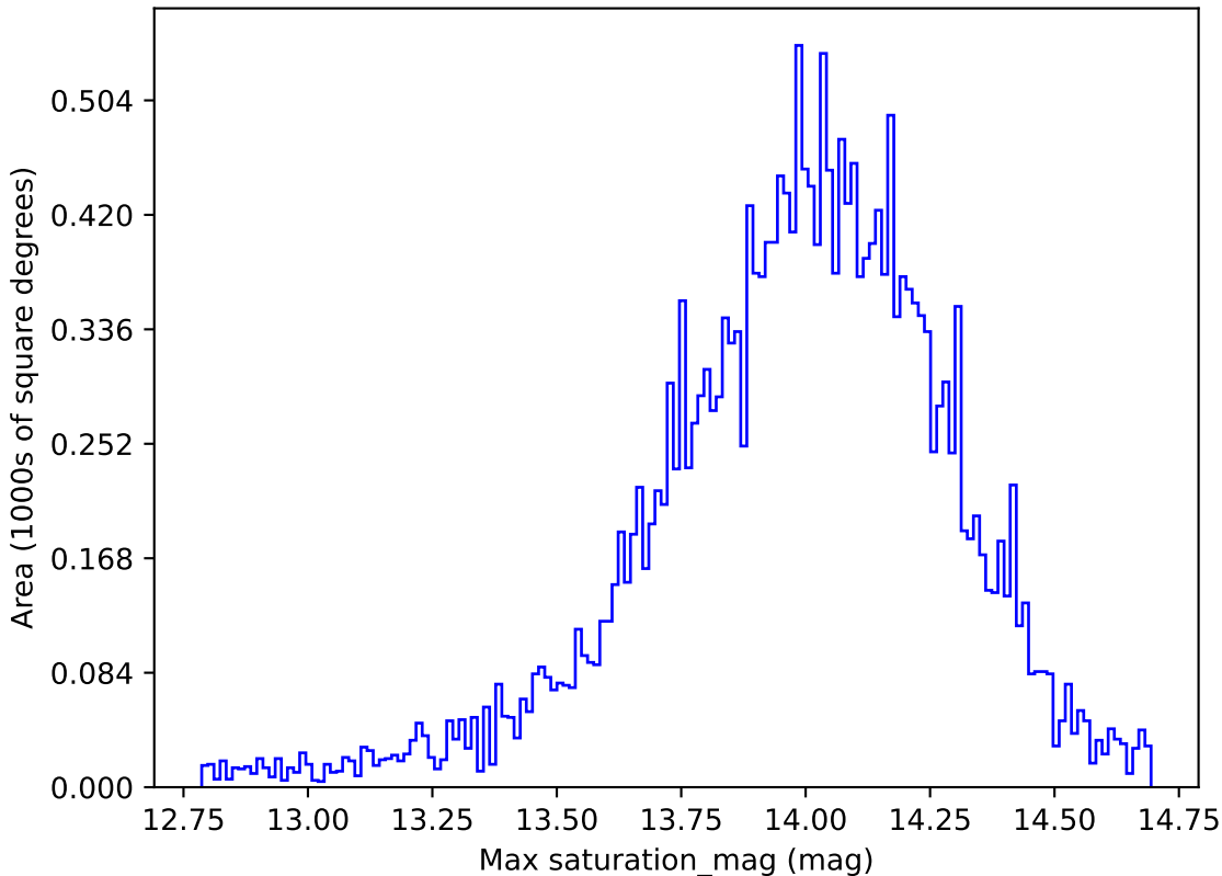
ddf_loaded_fl15_v3.4_10yrs All sky u band: Max saturation_mag
