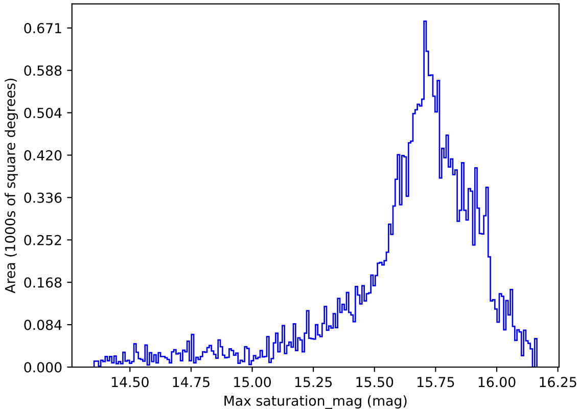
ddf_loaded_fl15_v3.4_10yrs All sky r band: Max saturation_mag
