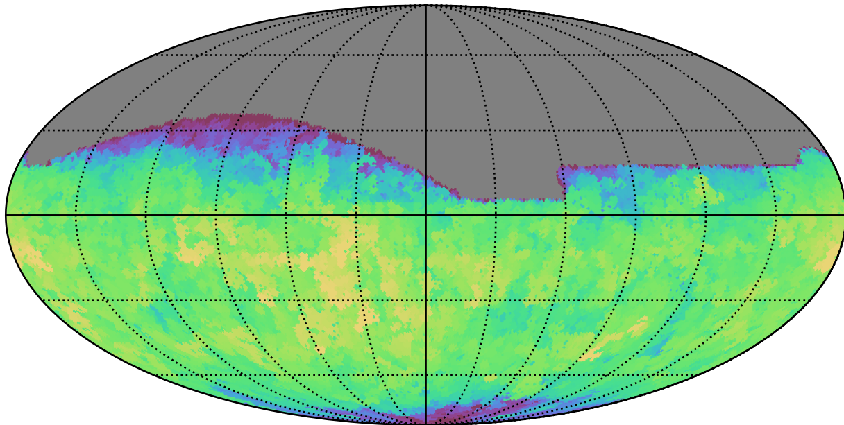
ddf_loaded_fl15_v3.4_10yrs All sky g band: Max saturation_mag
