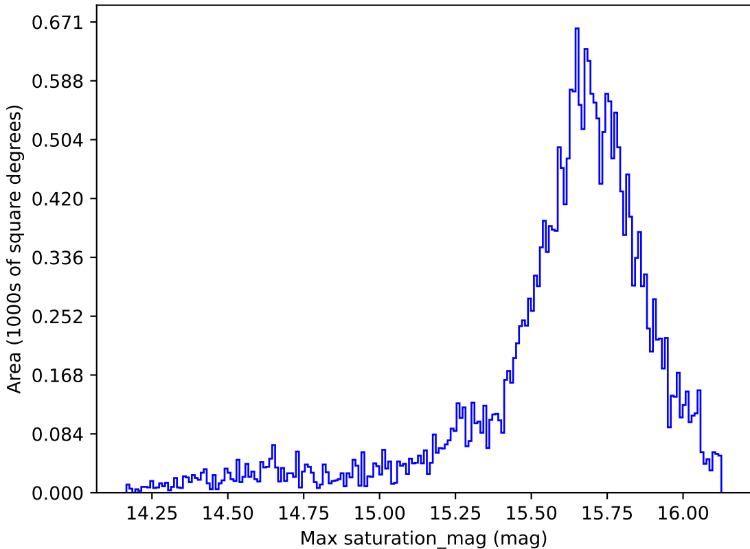
ddf_loaded_fl15_v3.4_10yrs All sky g band: Max saturation_mag
