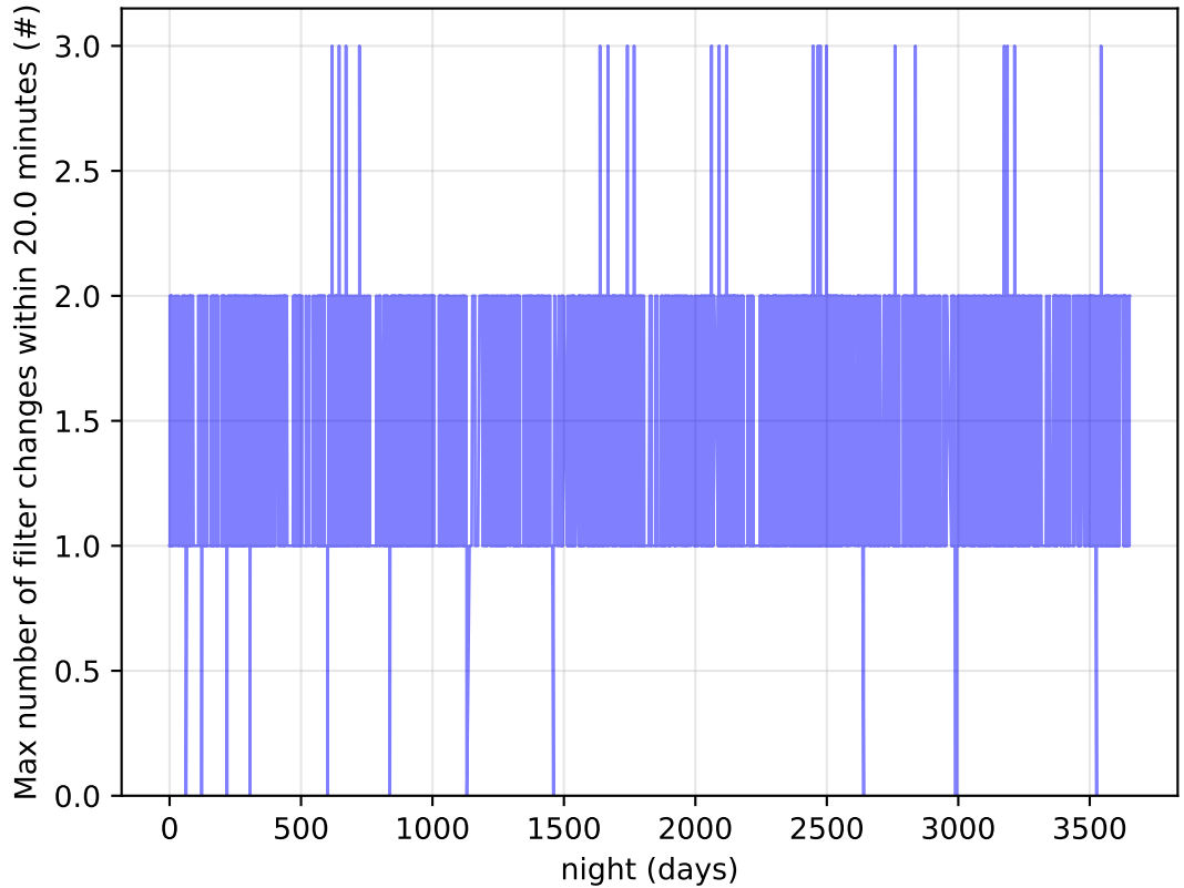
ddf_loaded_fl15_v3.4_10yrs Per Night: Max number of filter changes within 20.0 minutes
