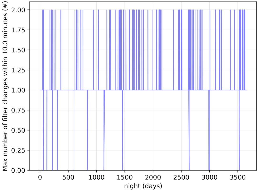
ddf_loaded_fl15_v3.4_10yrs Per Night: Max number of filter changes within 10.0 minutes
