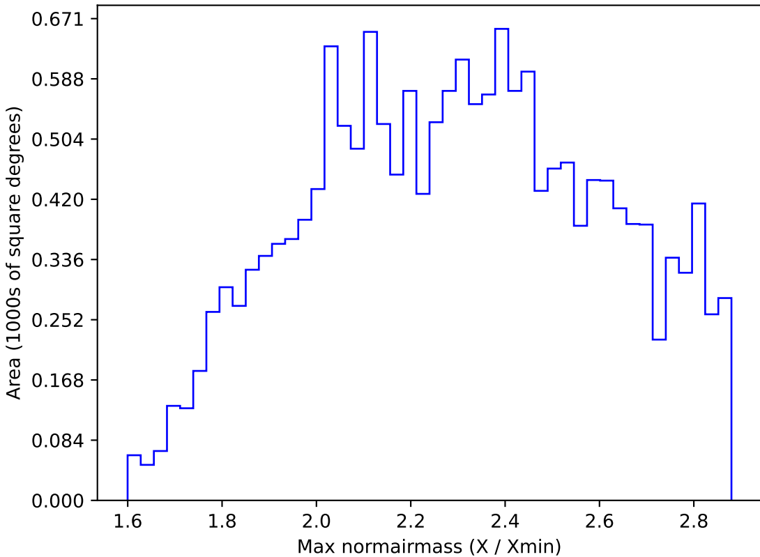
ddf_loaded_fl15_v3.4_10yrs WFD z band: Max normairmass
