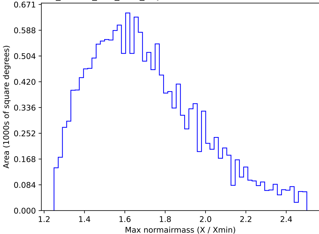
ddf_loaded_fl15_v3.4_10yrs WFD u band: Max normairmass
