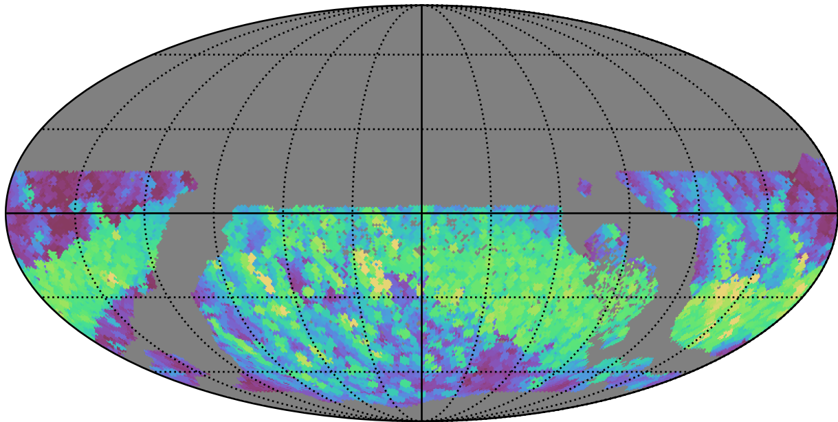
ddf_loaded_fl15_v3.4_10yrs WFD r band: Max normairmass
