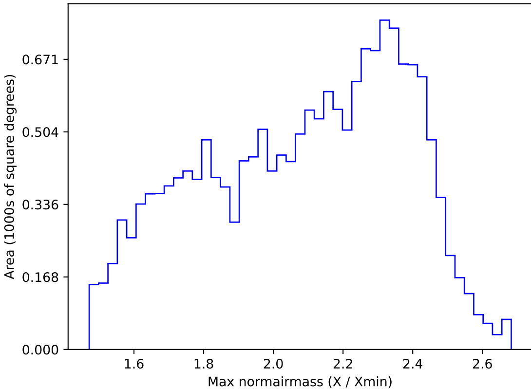
ddf_loaded_fl15_v3.4_10yrs WFD r band: Max normairmass
