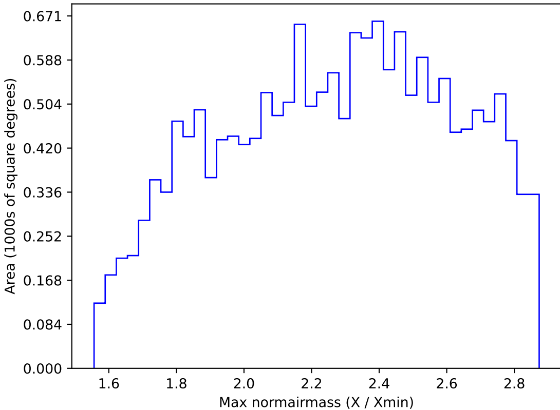
ddf_loaded_fl15_v3.4_10yrs WFD i band: Max normairmass
