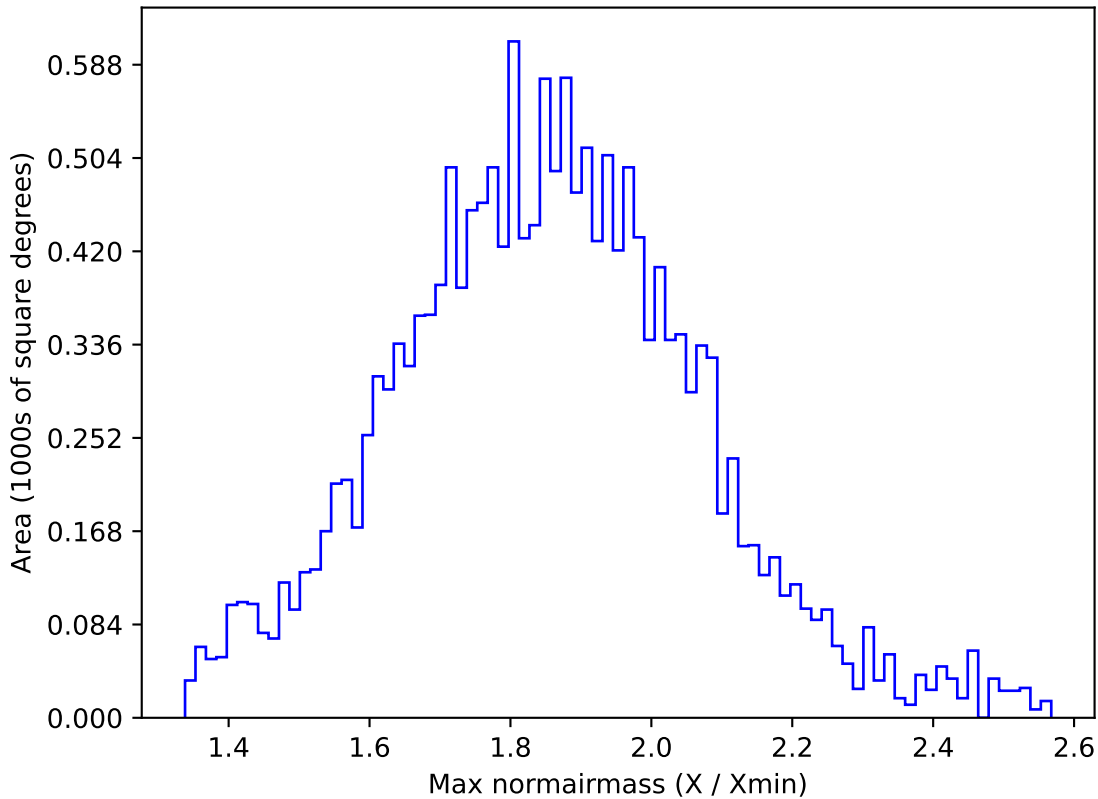
ddf_loaded_fl15_v3.4_10yrs WFD g band: Max normairmass
