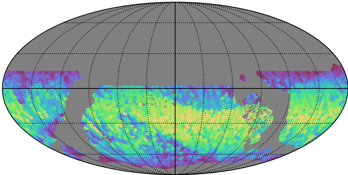
ddf_loaded_fl15_v3.4_10yrs WFD all bands: Max normairmass
