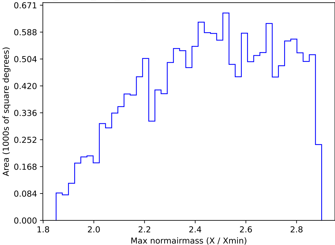
ddf_loaded_fl15_v3.4_10yrs WFD all bands: Max normairmass
