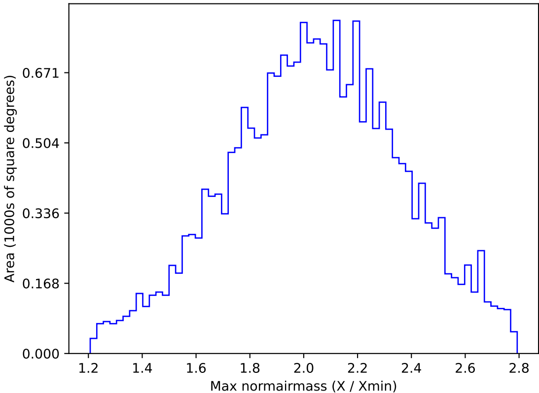
ddf_loaded_fl15_v3.4_10yrs All sky y band: Max normairmass
