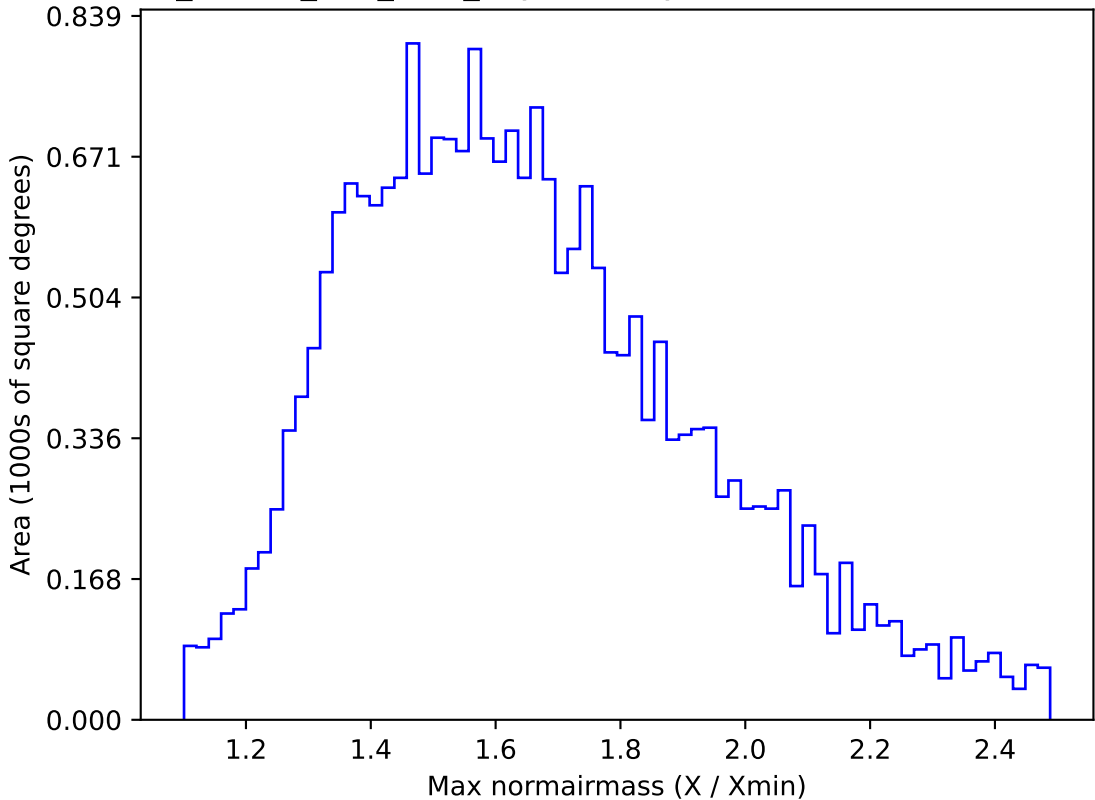
ddf_loaded_fl15_v3.4_10yrs All sky u band: Max normairmass
