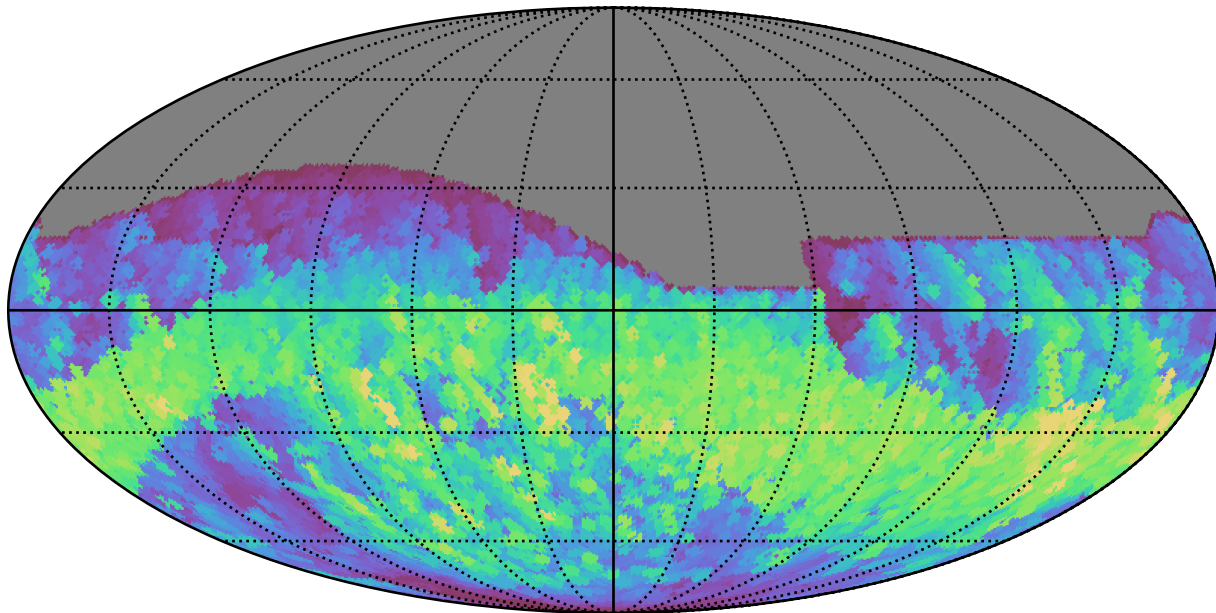
ddf_loaded_fl15_v3.4_10yrs All sky r band: Max normairmass
