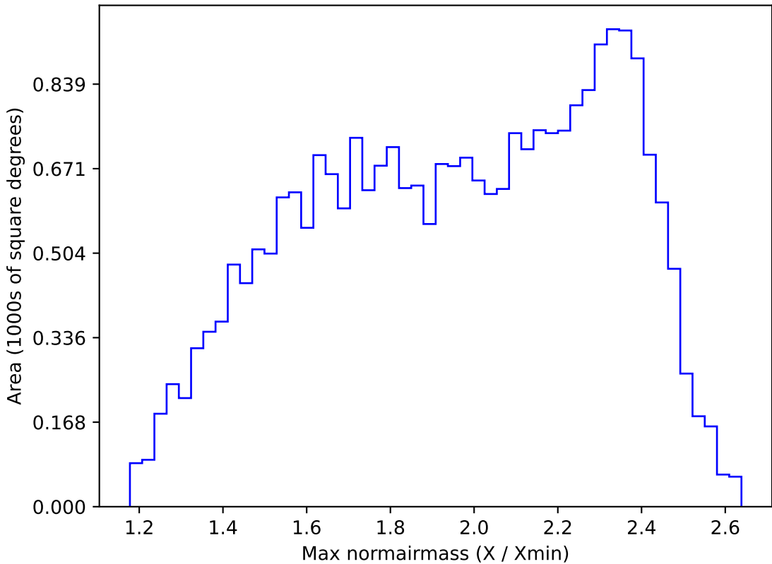
ddf_loaded_fl15_v3.4_10yrs All sky r band: Max normairmass
