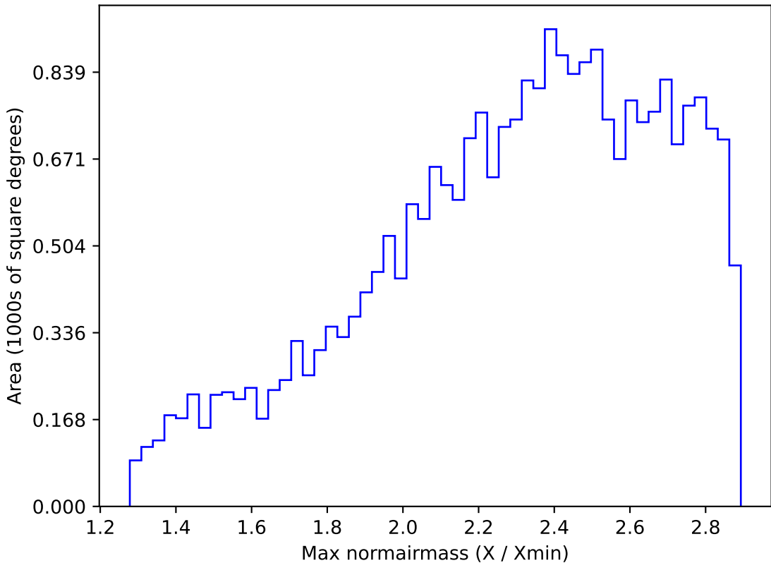
ddf_loaded_fl15_v3.4_10yrs All sky all bands: Max normairmass
