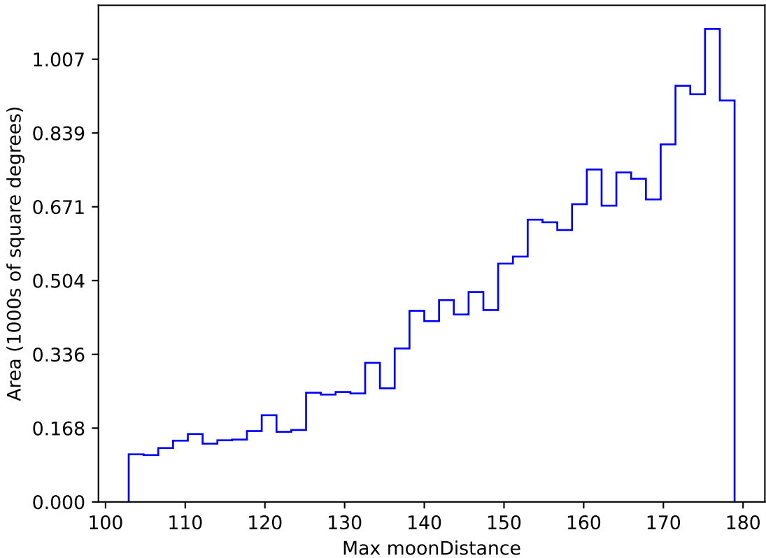
ddf_loaded_fl15_v3.4_10yrs WFD z band: Max moonDistance
