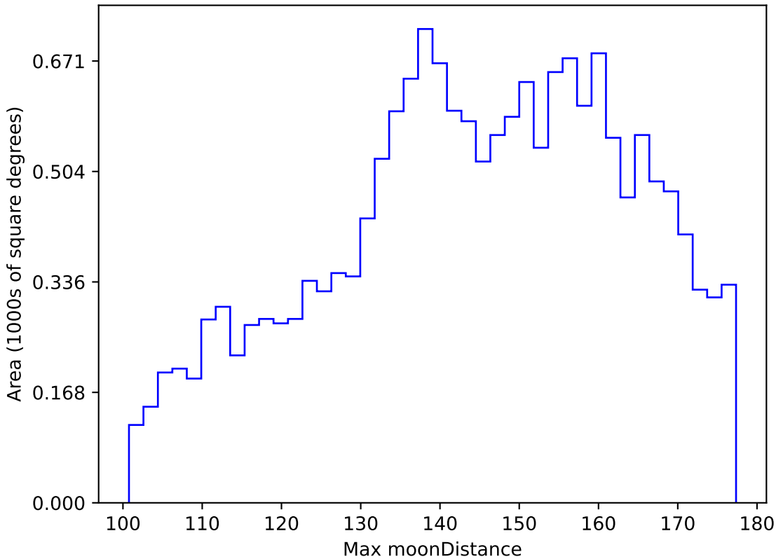
ddf_loaded_fl15_v3.4_10yrs WFD y band: Max moonDistance
