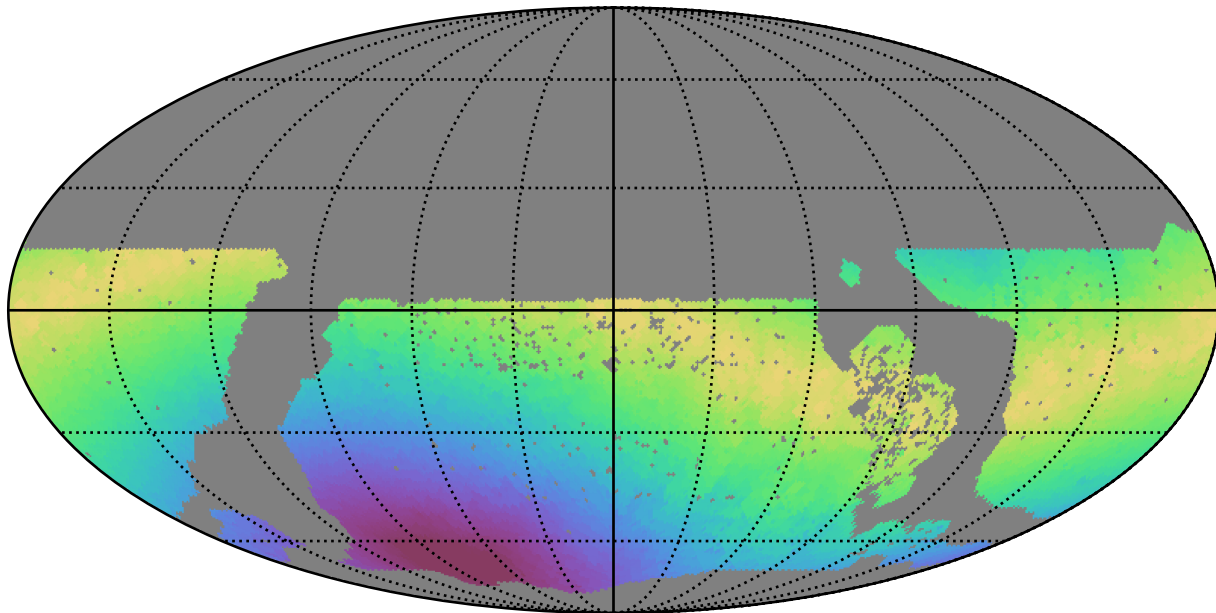
ddf_loaded_fl15_v3.4_10yrs WFD u band: Max moonDistance
