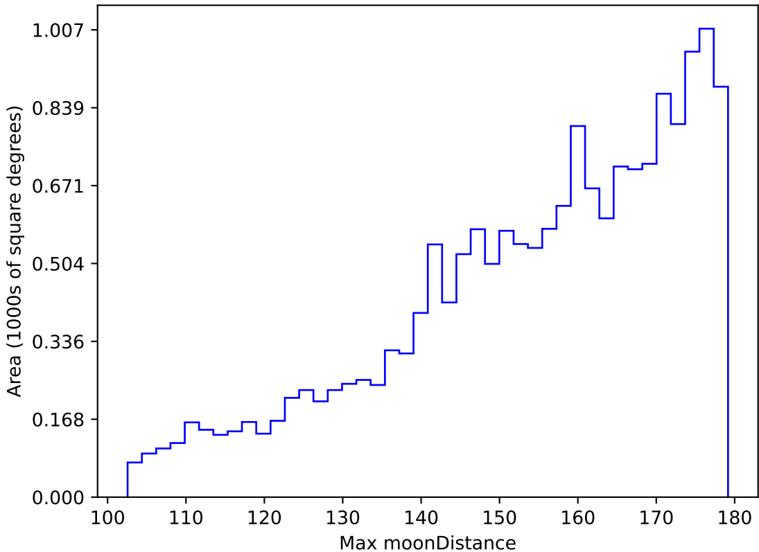
ddf_loaded_fl15_v3.4_10yrs WFD u band: Max moonDistance
