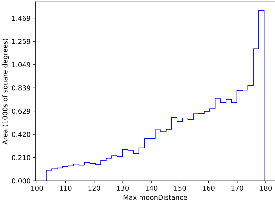
ddf_loaded_fl15_v3.4_10yrs WFD r band: Max moonDistance
