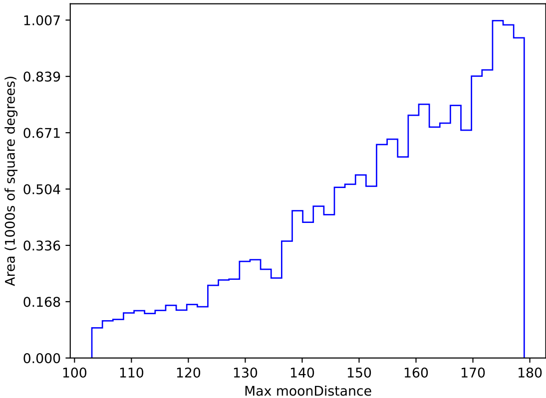
ddf_loaded_fl15_v3.4_10yrs WFD g band: Max moonDistance
