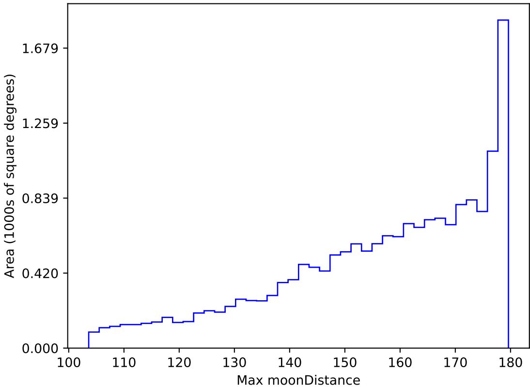
ddf_loaded_fl15_v3.4_10yrs WFD all bands: Max moonDistance
