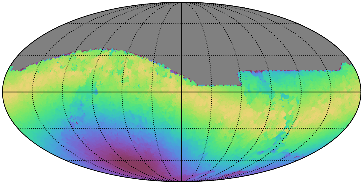
ddf_loaded_fl15_v3.4_10yrs All sky z band: Max moonDistance
