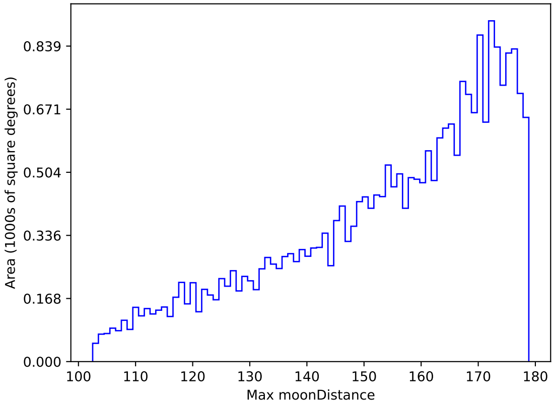
ddf_loaded_fl15_v3.4_10yrs All sky z band: Max moonDistance
