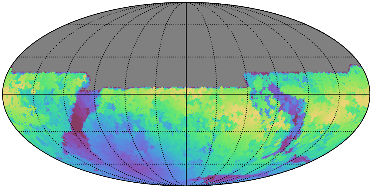
ddf_loaded_fl15_v3.4_10yrs All sky y band: Max moonDistance
