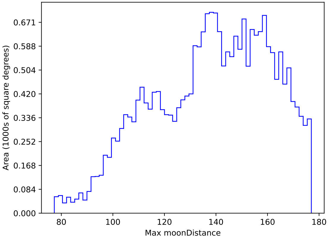
ddf_loaded_fl15_v3.4_10yrs All sky y band: Max moonDistance
