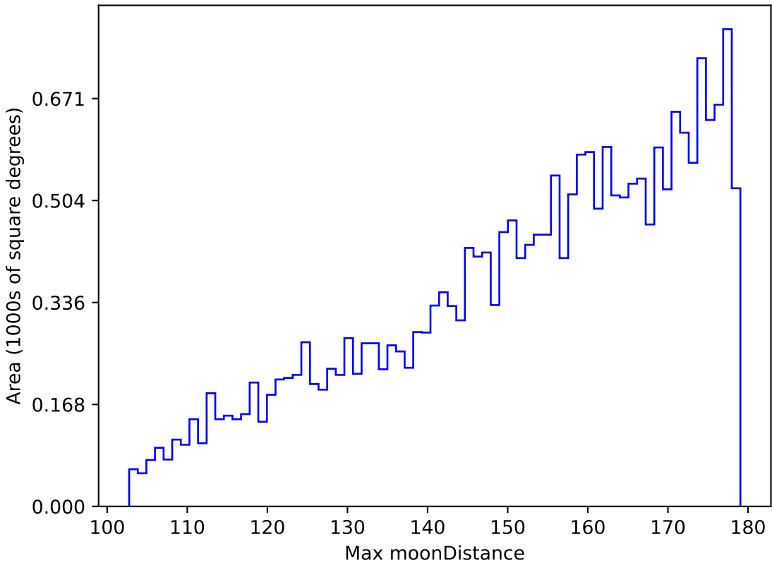
ddf_loaded_fl15_v3.4_10yrs All sky u band: Max moonDistance
