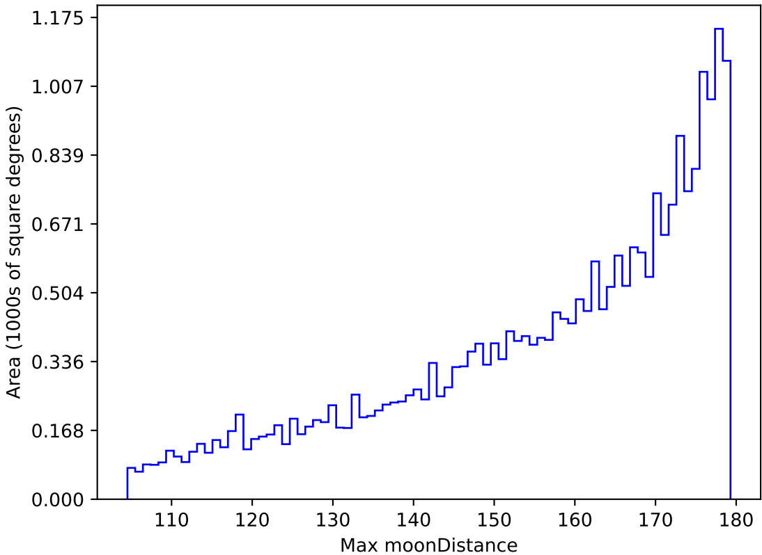
ddf_loaded_fl15_v3.4_10yrs All sky r band: Max moonDistance
