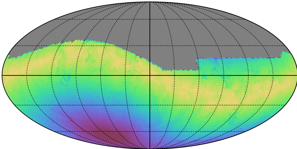
ddf_loaded_fl15_v3.4_10yrs All sky g band: Max moonDistance
