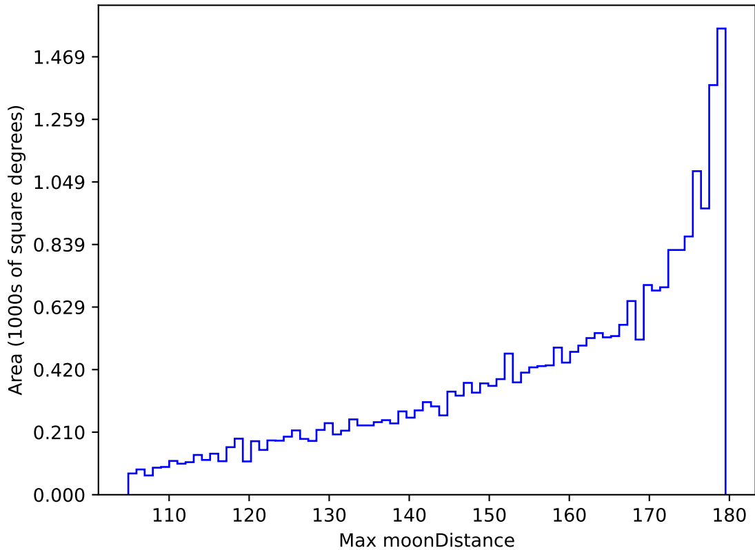
ddf_loaded_fl15_v3.4_10yrs All sky all bands: Max moonDistance
