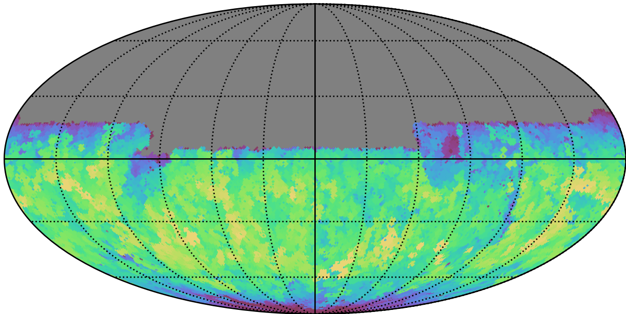
ddf_loaded_fl15_v3.4_10yrs Yr 1 y band: Max fiveSigmaDepth
