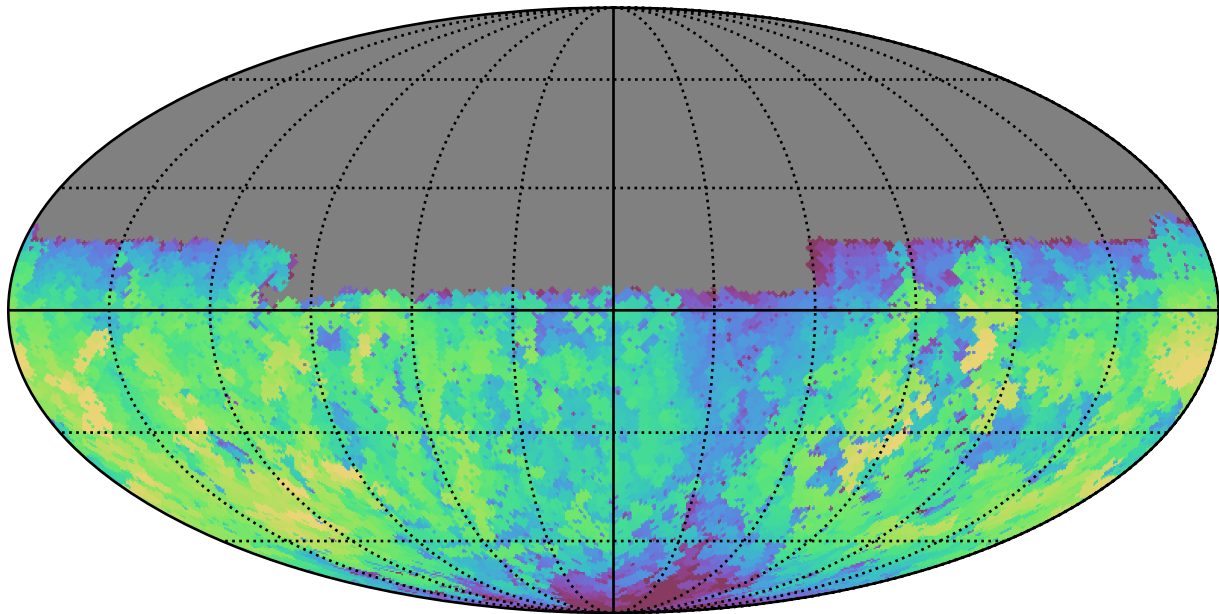
ddf_loaded_fl15_v3.4_10yrs Yr 1 u band: Max fiveSigmaDepth
