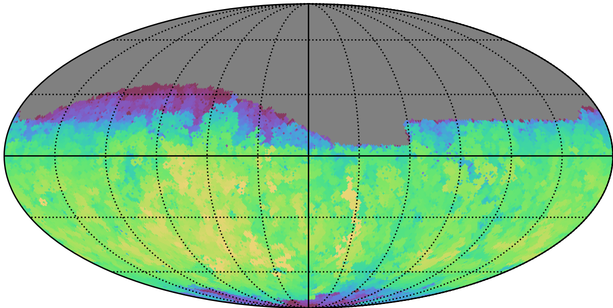
ddf_loaded_fl15_v3.4_10yrs Yr 1 r band: Max fiveSigmaDepth
