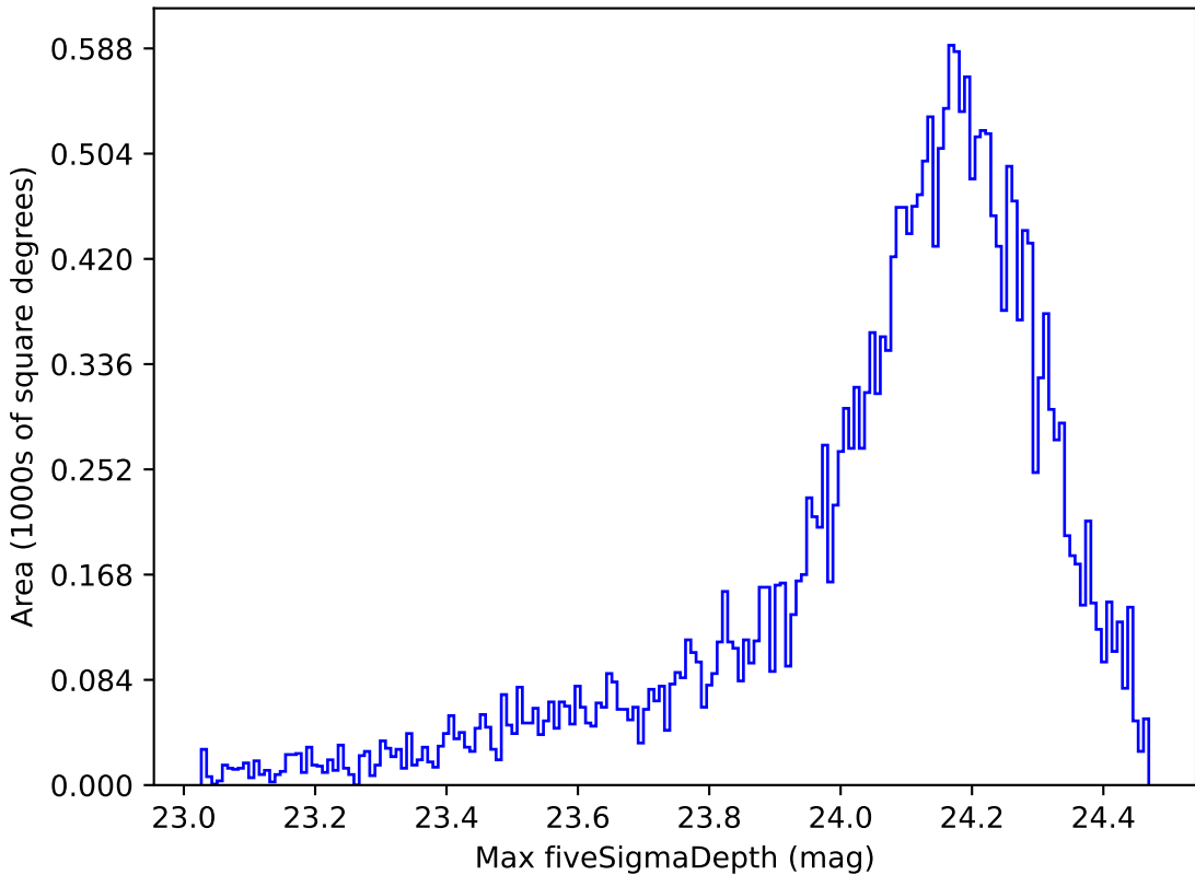
ddf_loaded_fl15_v3.4_10yrs Yr 1 i band: Max fiveSigmaDepth
