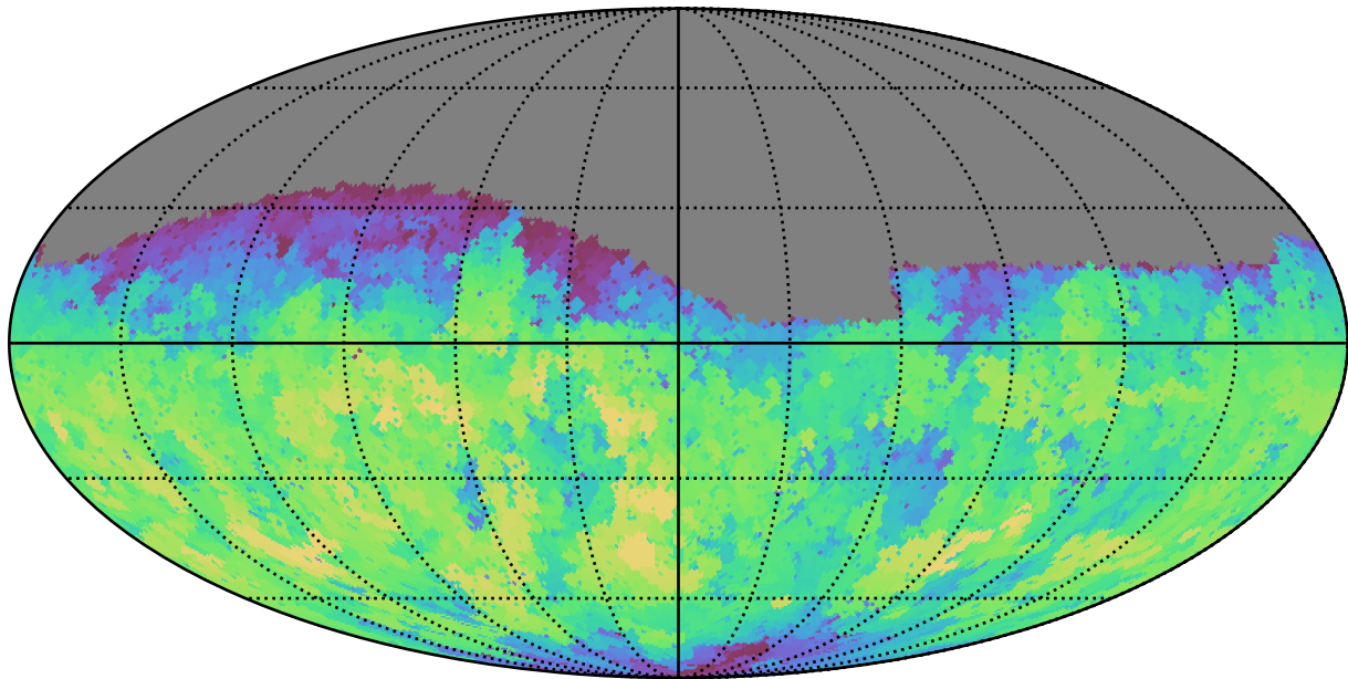
ddf_loaded_fl15_v3.4_10yrs Yr 1 g band: Max fiveSigmaDepth
