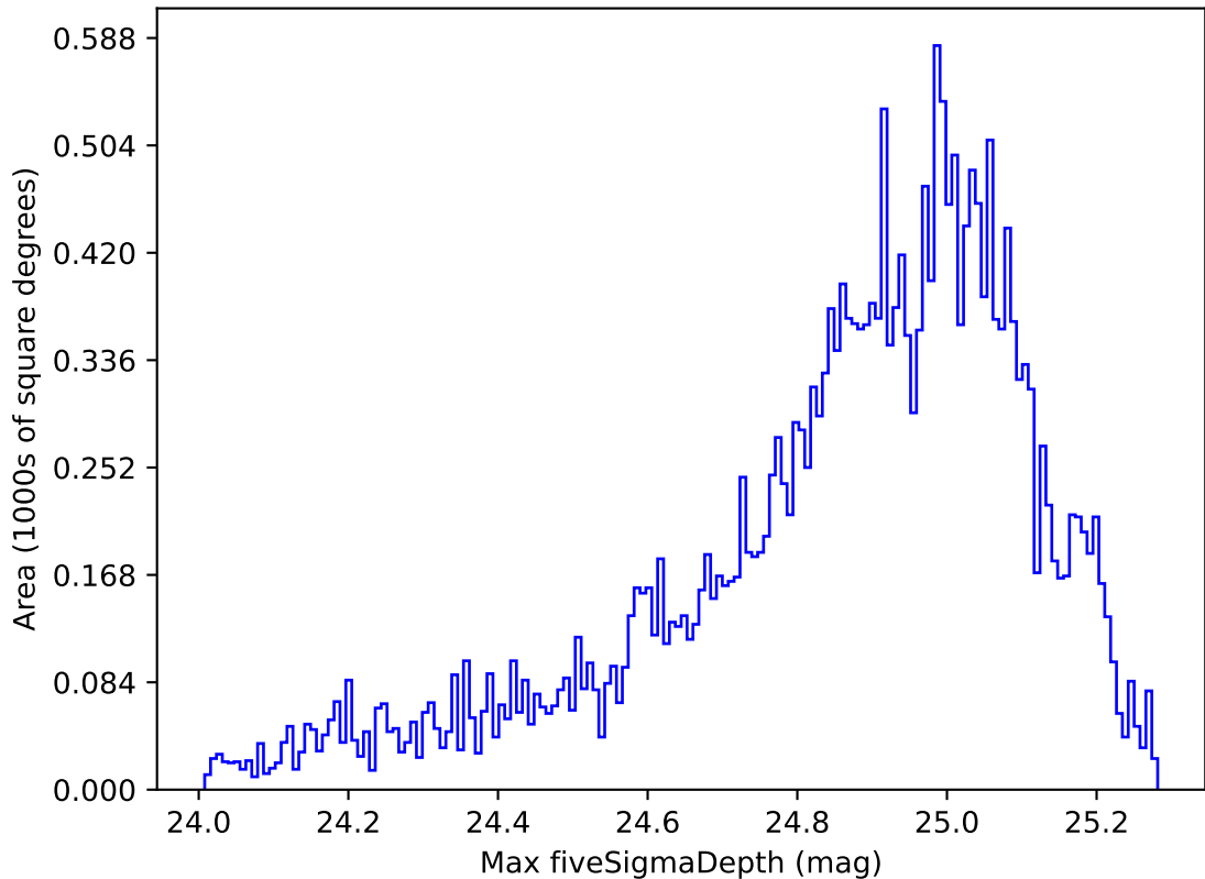
ddf_loaded_fl15_v3.4_10yrs Yr 1 g band: Max fiveSigmaDepth
