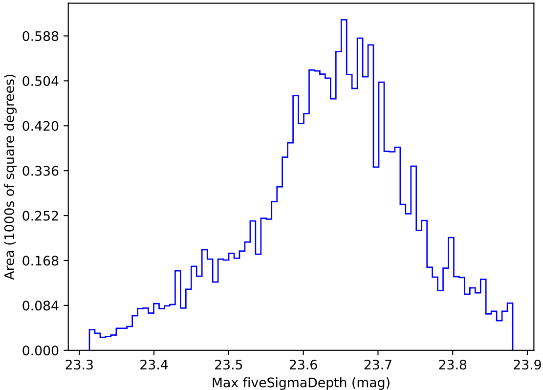
ddf_loaded_fl15_v3.4_10yrs WFD z band: Max fiveSigmaDepth
