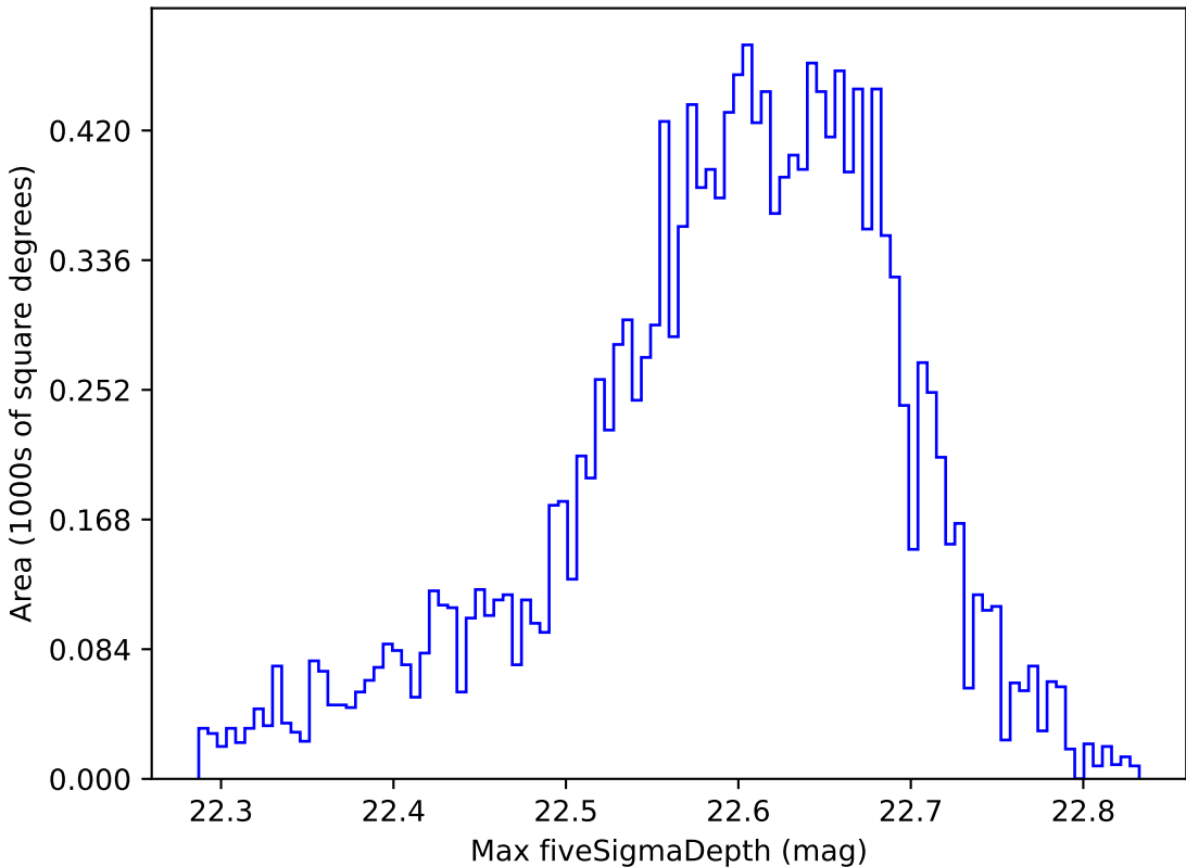
ddf_loaded_fl15_v3.4_10yrs WFD y band: Max fiveSigmaDepth
