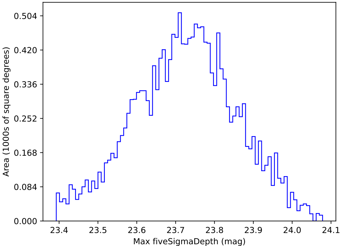
ddf_loaded_fl15_v3.4_10yrs WFD u band: Max fiveSigmaDepth
